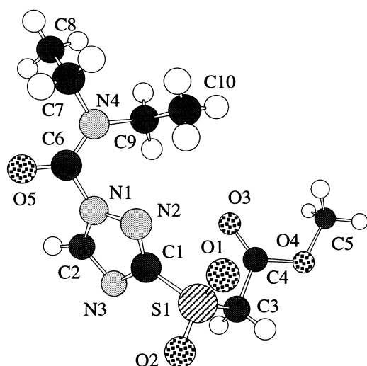
Fig. 3. Crystal structure of 5a by X-ray analysis.
