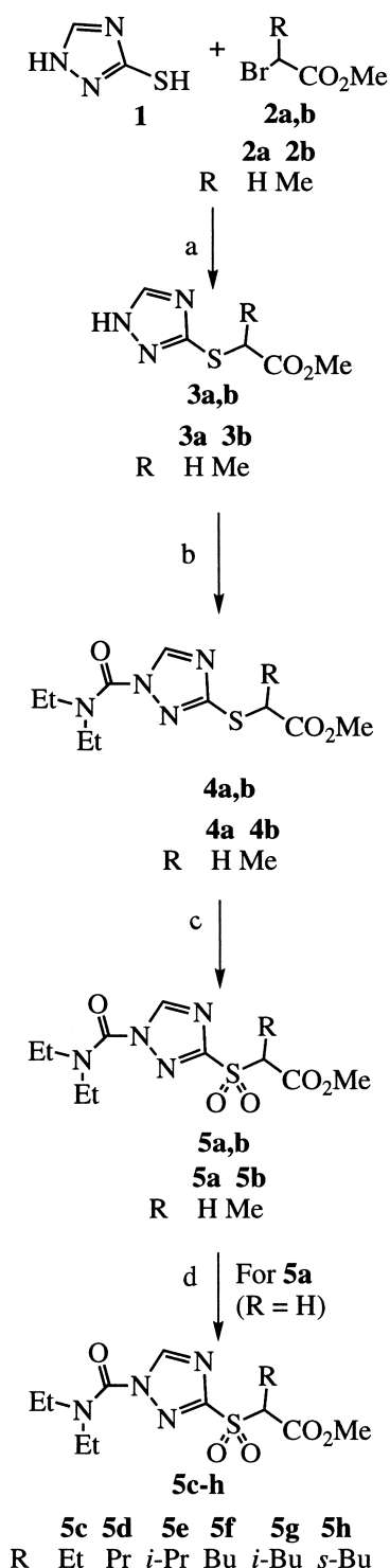
Scheme 1. Reagents and conditions: (a) 2a,b , \text{K}_2\text{CO}_3 , MeCN, reflux. (b) \text{Et}_2\text{NCOCl} , \text{K}_2\text{CO}_3 , MeCN, 50–60 °C. (c) m CPBA, \text{CHCl}_3 , 0 °C. (d) RI, NaH, DMF, rt.
