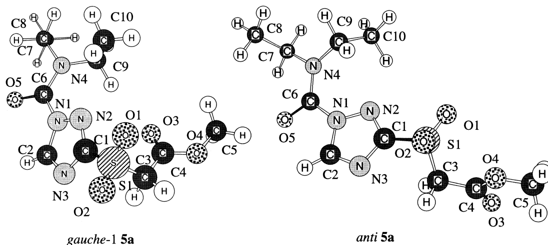
Fig. 4. Molecular structure of 5a simulated by AM1 level calculations.
